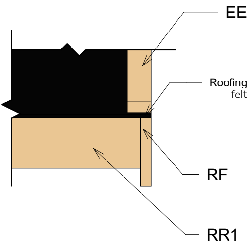
3) Roof Reinforcement
