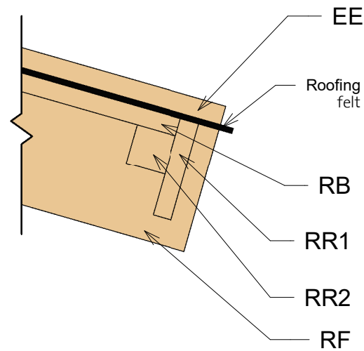
3) Roof Reinforcement
